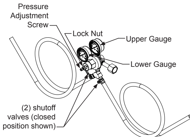
Figure 40 (Regulator for Double Dispense Tower)
